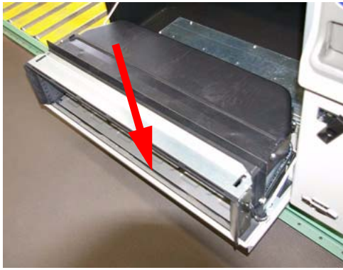
Install 4614027 SEAL on the inside top lip of delivery bin.
